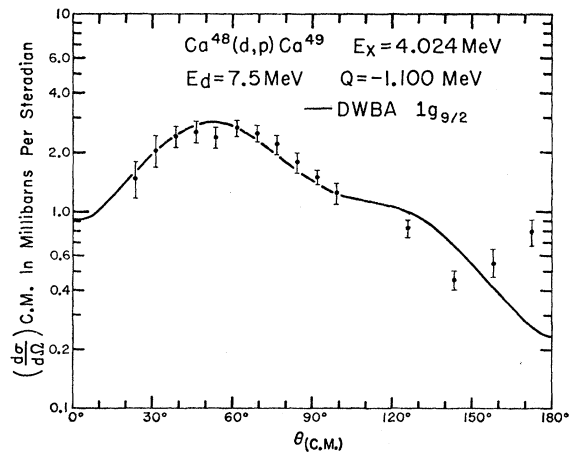
FIG. 7. Angular distribution of protons leaving \text{Ca}^{49} in its 4.024-MeV level.
