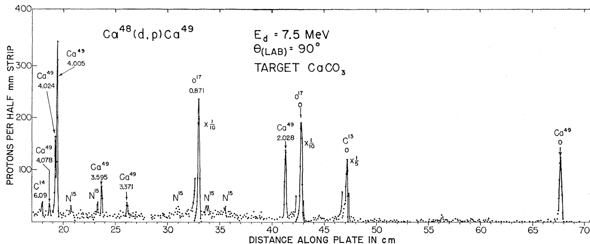
FIG. 1. Momentum spectrum of protons from the \text{Ca}^{48}(d,p)\text{Ca}^{49} reaction at a laboratory angle of 90 deg.
