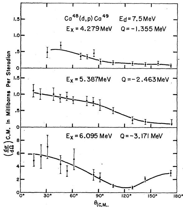
FIG. 9. Angular distributions of protons to the 4.279-, 5.387-, and 6.095-MeV levels of \text{Ca}^{49} . The solid curves are drawn through the experimental data.
