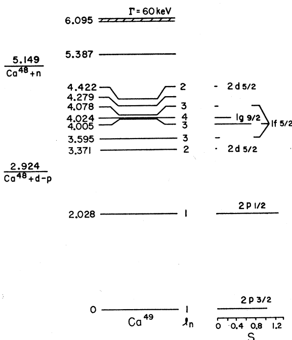
FIG. 10. Energy-level diagram of Ca 49 , with spectroscopic factors for the Ca 48 ( d,p )Ca 49 reaction shown.
