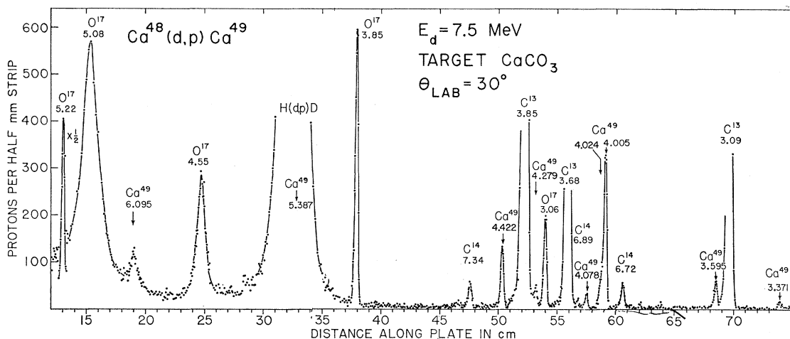
FIG. 3. Momentum spectrum of protons from the Ca 48 ( d,p )Ca 49 reaction at a laboratory angle of 30 deg.
